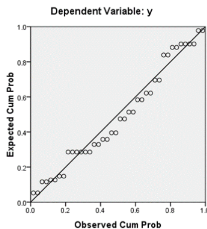
Gambar 4. Normal Probability Plot
